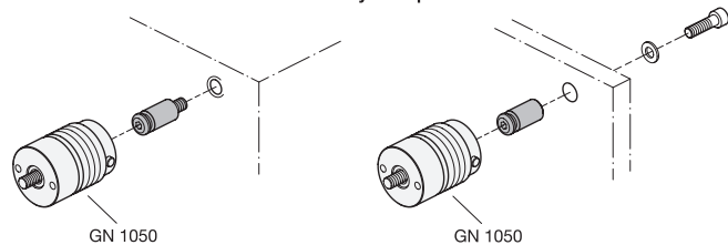
Assembly examples
