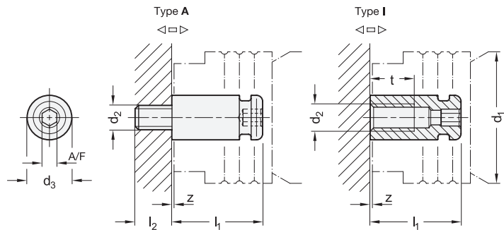
Assembly examples
